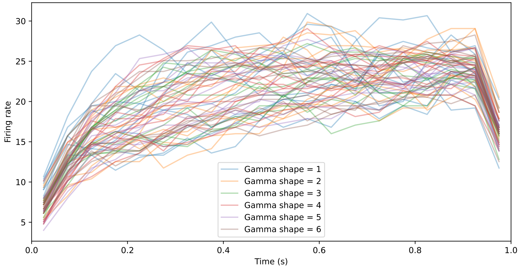
Ramp-like PSTHs for each gamma emission shape
